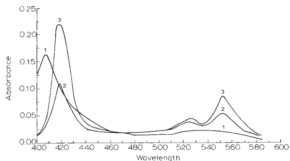
Fig. 2. Electronic absorption spectra of oxidized (1), lactate reduced (2), and dithionate reduced (3) Desulfovibrio desulfuricans lactate dehydrogenase (sp. act. 525).
