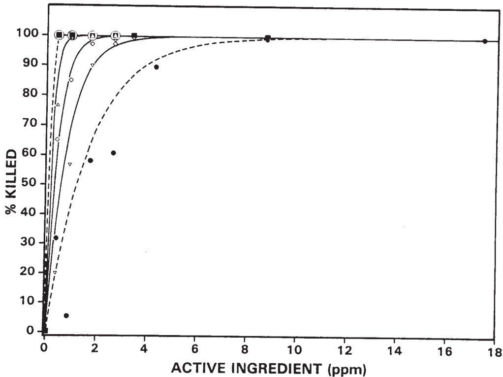
Fig. 2. The effect of methylchloroisothiazolone biocide on Legionella pneumophila in cooling tower water. The symbols are data recalculated from Table 1 and the curves were calculated from eqn. 3 (in Results). Symbols (also see Table 2): \circ , \Delta , \nabla , pH 8.0 after 24, 6 and 3 h of contact, respectively; \blacksquare , \diamond , \bullet , pH 6.7 after 24, 6 and 3 h of contact, respectively.
